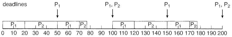
Figure 19.8 Rate-monotonic scheduling.
