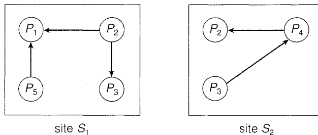
Figure 18.3 Two local wait-for graphs.
